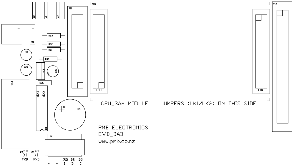
EVB_3A3 Top Overlay
