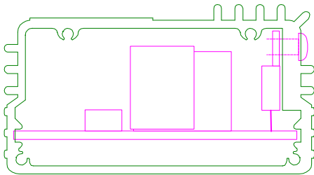
extrusion end view scale 1:1
